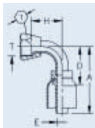
OTC Fitting
