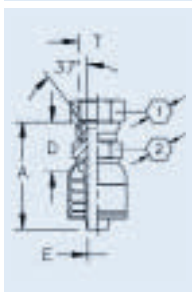
TTC Fitting
