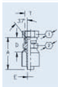
OTC Fitting
