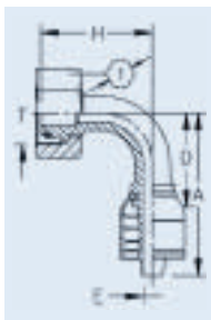
TTC Fitting
