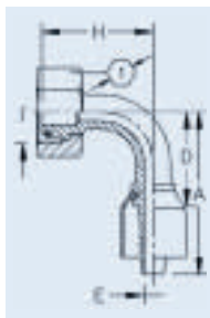
OTC Fitting
