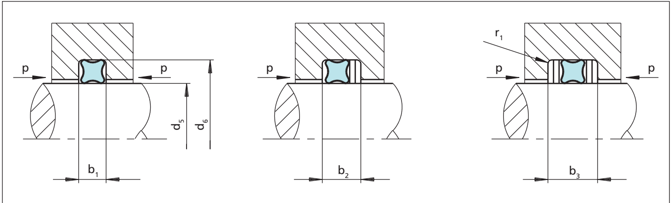
Figure 17 Installation drawing
